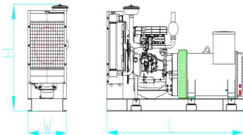
Open Type (Standard Configuration) Overall Size: 1750×750 ×1230mm(L*W*H) Weight: 880kgs
