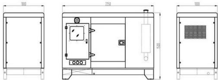
Soundproof Type Overall size: 2250× 1000×1550mm(L*W*H) Weight: 1280kgs
