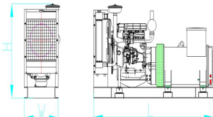
Open Type (Standard Configuration) Overall Size: 1510×750 ×1120mm(L*W*H) Weight: 630kgs
